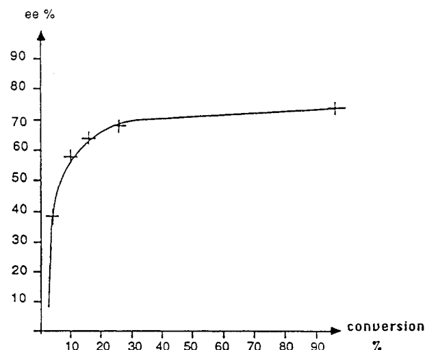
Figure 4. Asymmetric synthesis of (-)-I with a chiral catalyst (0.05 equiv) prepared from EtAlCl 2 and (S)-3a (1:1). Reaction performed in CH 2 Cl 2 at -78 °C.
